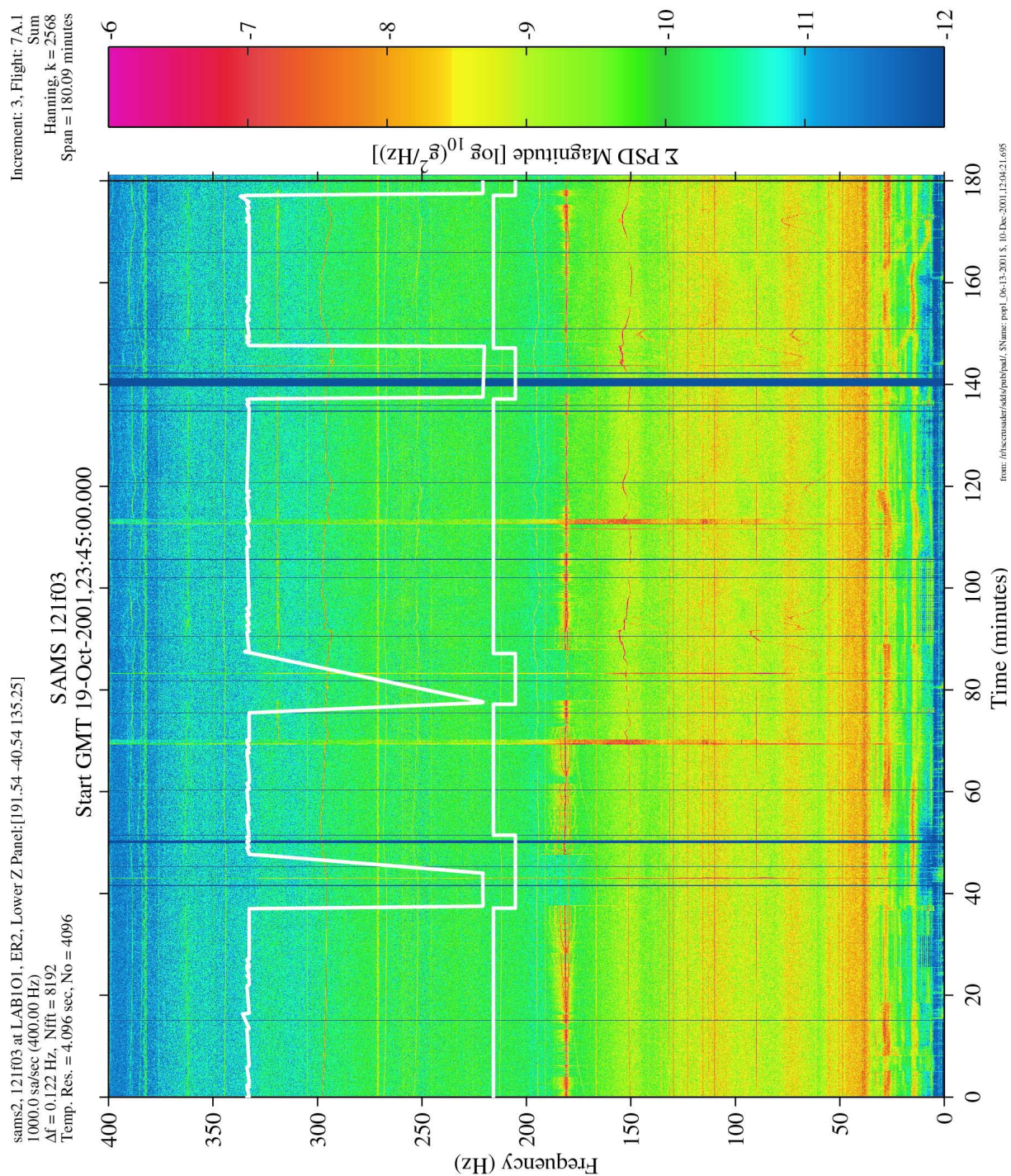
Figure 6-41 Spectrogram of AAA Fan (De)activations (121f03)
