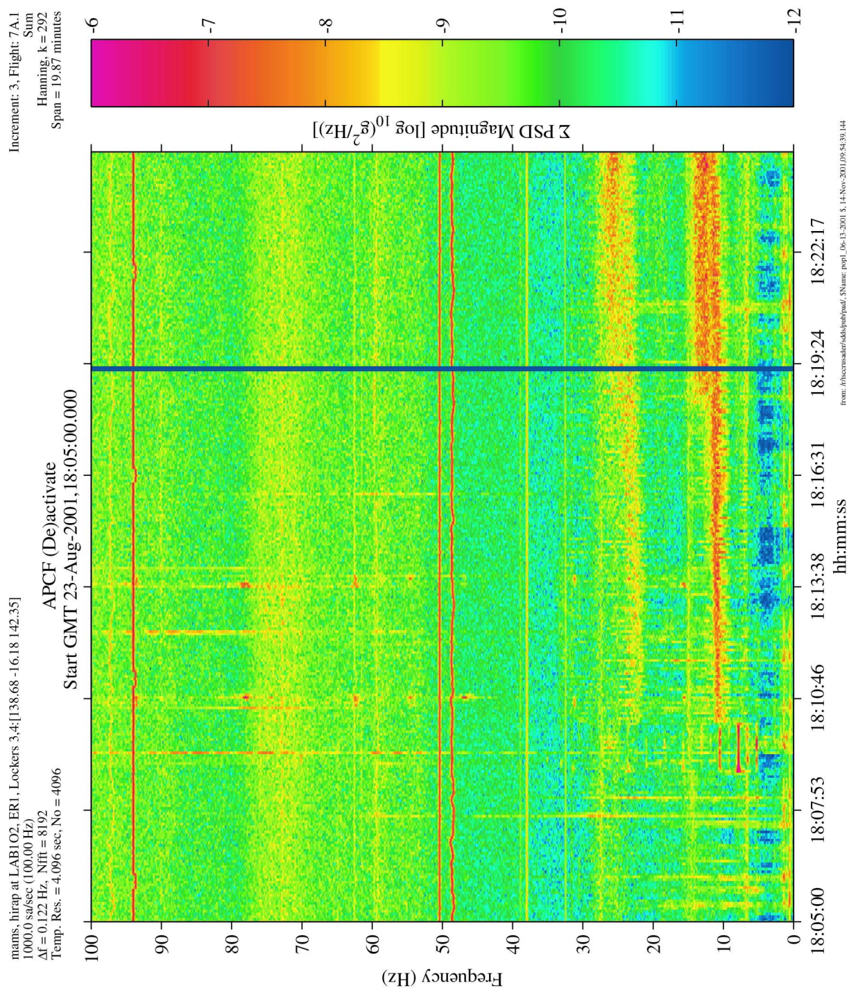
Figure 6-64 Spectrogram of [Not Apparent] APCF Deactivation/Activation (HiRAP)
