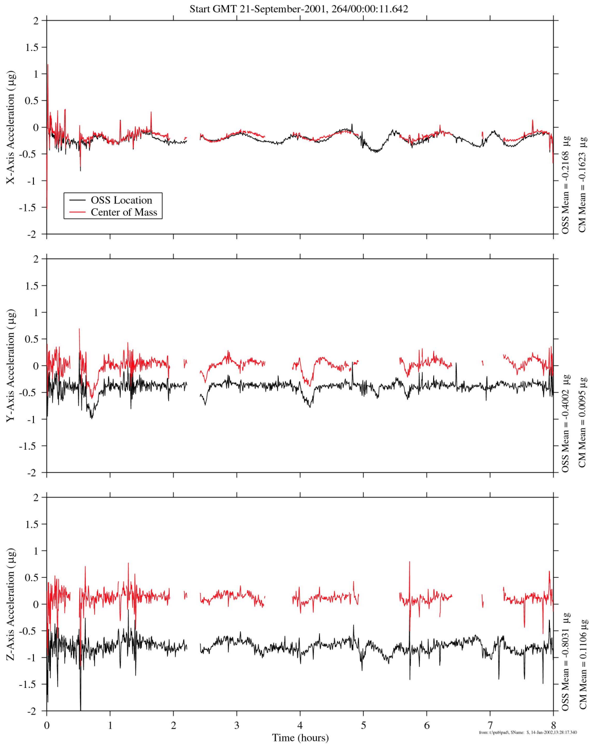
Figure 6-1 Time Series of Quasi-steady Vector During TEA (OSS)
