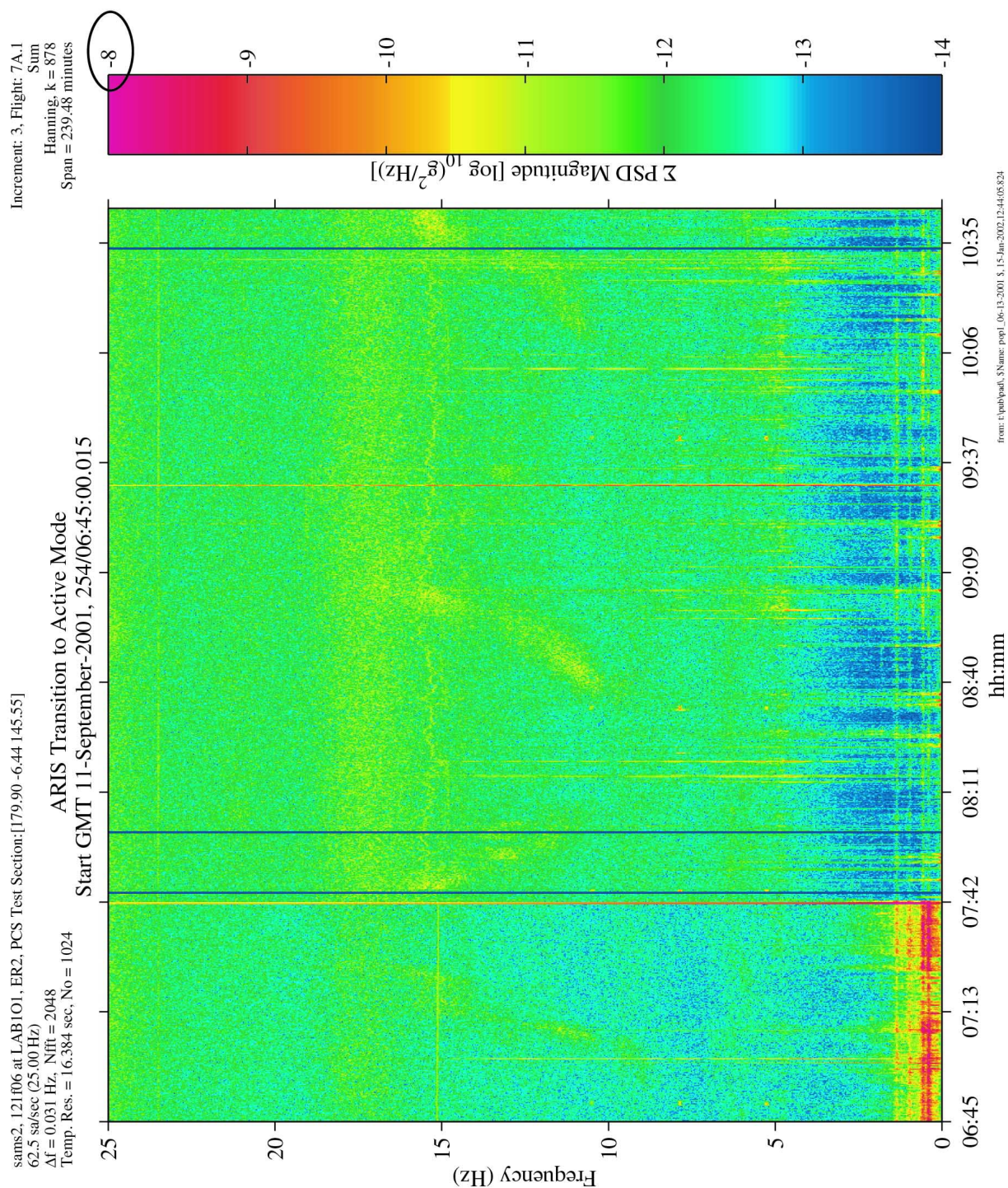
Figure 6-56 Spectrogram of ARIS Transition to Active Mode Zoom (121f06)
