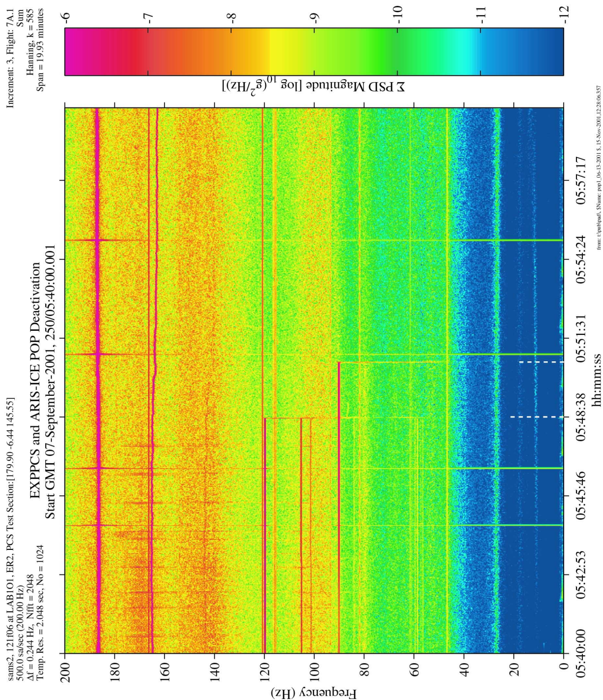
Figure 6-63 Spectrogram of EXPPCS and ARIS-ICE POP Deactivation (121f06)
